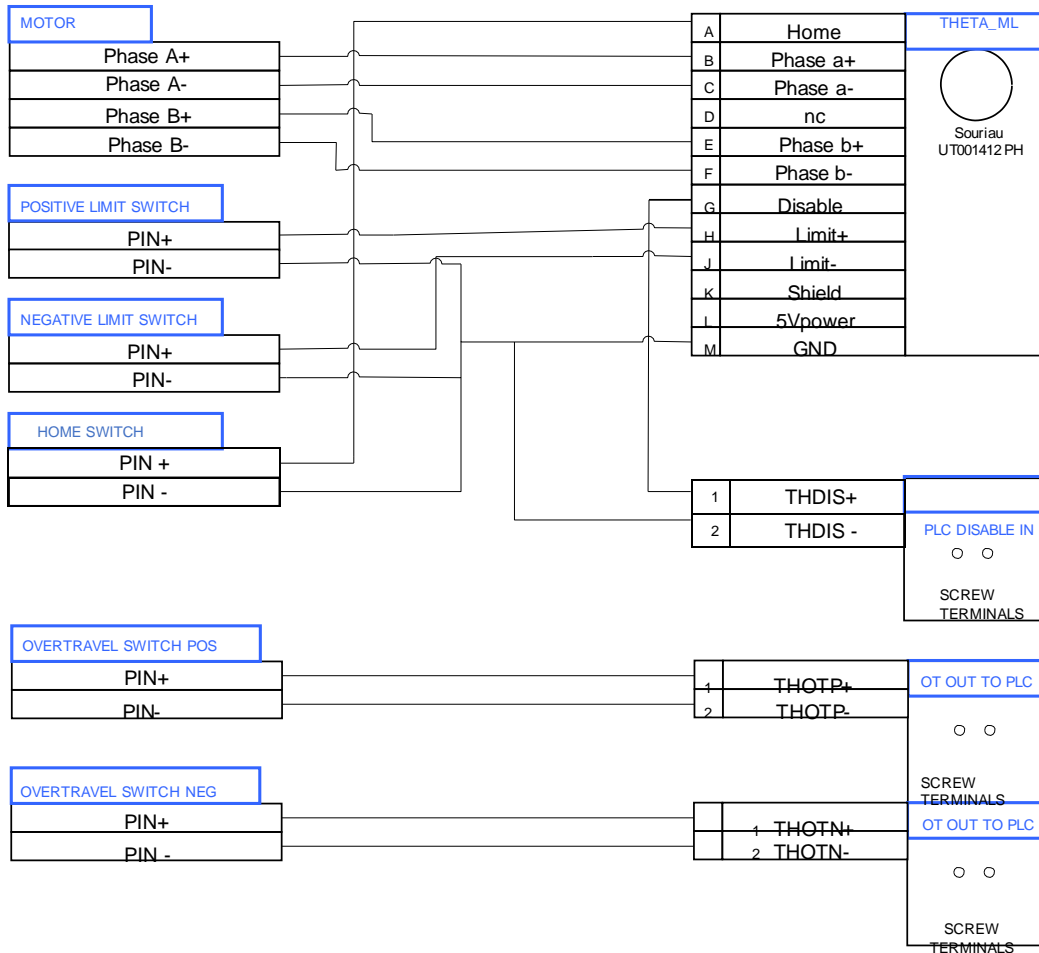
Figure 10. Interface box wiring diagram for overtravel PLC disabled axis
