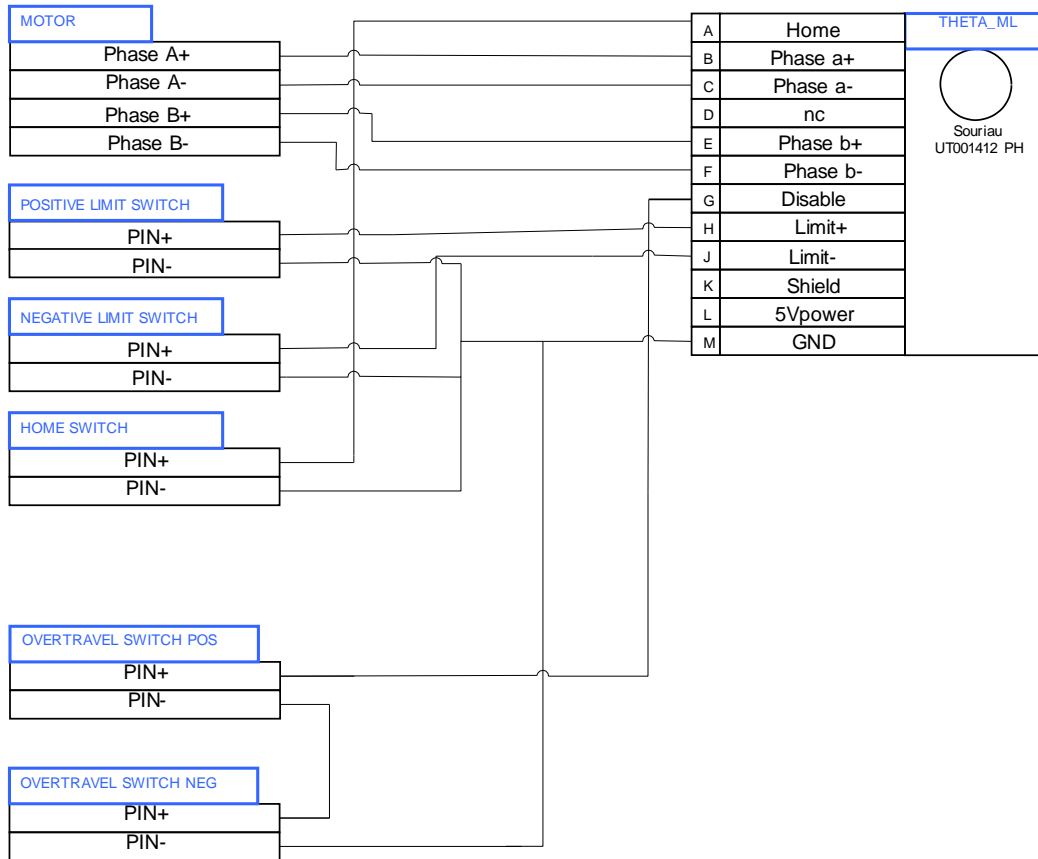
Figure 11. Interface box wiring diagram for overtravel disabled axis without external hardware
